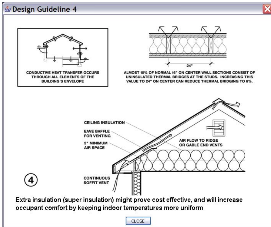
Fig.10: Design Guideline Sketches: If you click on the ID number of any guideline you will get a Sketch further explaining more about how it affects the architectural form of the building.
