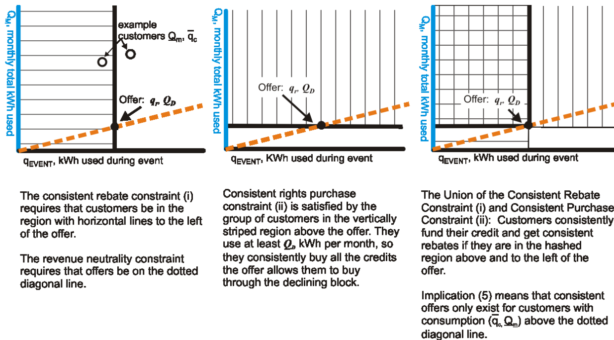
Figure 4: Visualizing constraints 1-3.
